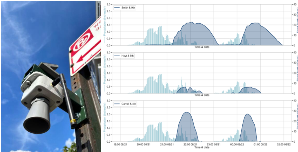
Figure 1 A flood sensor employed by the FloodNet project, and an example of a recording during a flood event
