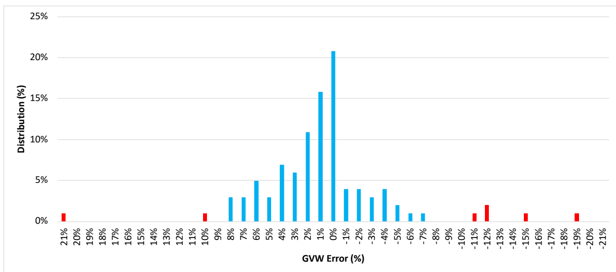
Figure 29: Distribution of GVW Errors
